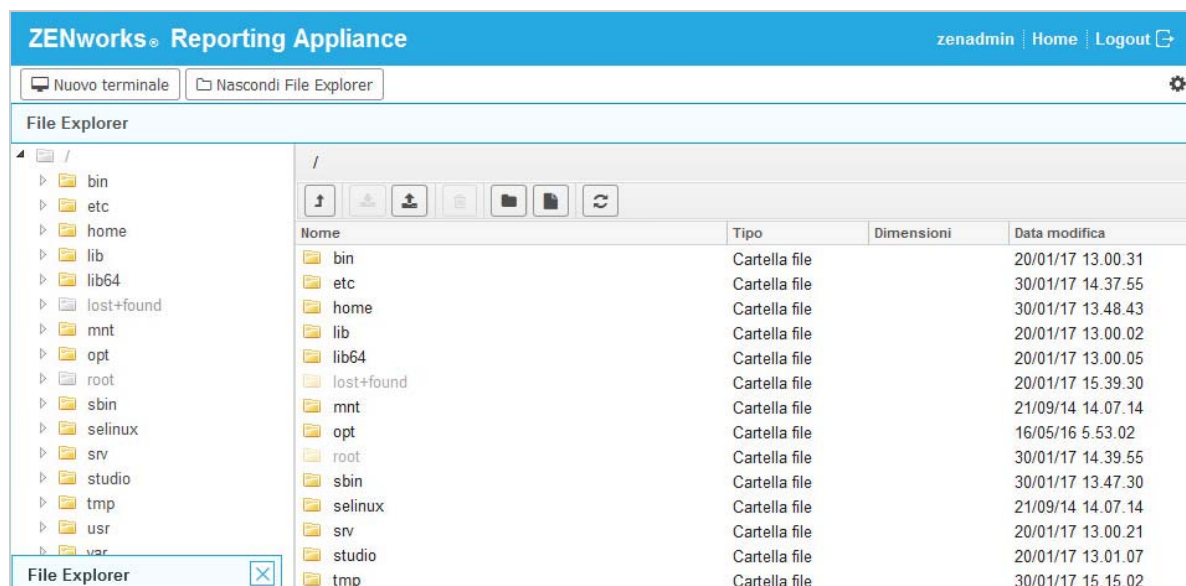
Figura 6-5 File Explorer
